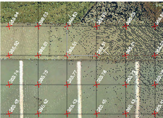
Points on a grid and intelligent SmartPick snaps provide a highly productive automated surveying tool used to create COGO points most typically used to generate a ground surface\TIN.
